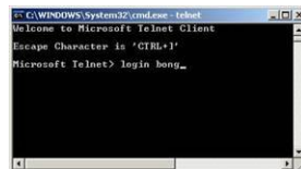
Unix PAM
